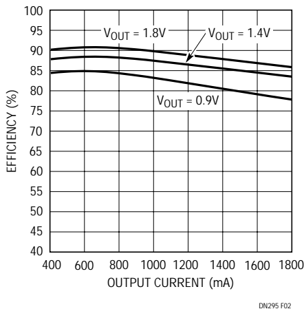
Figure 2. Efficiencies for the Circuit in Figure 1 where V IN = 3.3V
