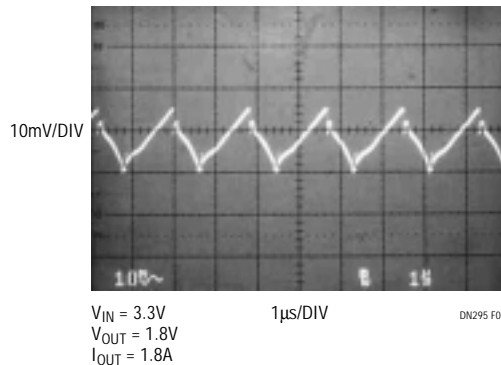
Figure 3. Output Voltage Ripple for the Circuit in Figure 1
