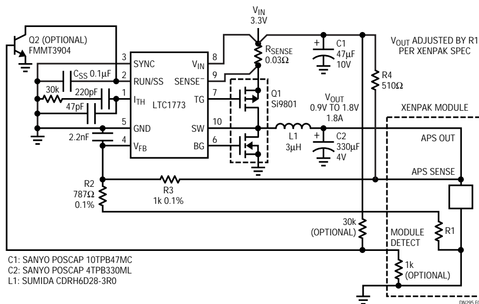
Figure 1. Adaptable Power Supply Using the LTC1773
